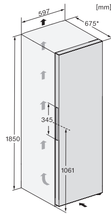
K4373DDws, K4373ED, FN4372E, FN4372D, installation sketch (footnote*) (installation drawings)
